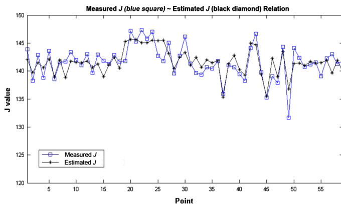
Fig. 5 Measured spin-coupling constant J (blue open square) and estimated J (black filled diamond) values generated using MATLAB
